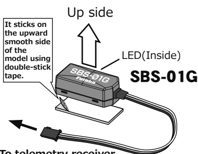
To telemetry receiver S.BUS2 port
